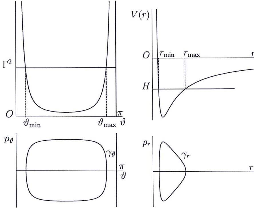
Figure 3.10 The construction of the cycles \gamma_\vartheta and \gamma_r for the problem of motion in a central field under the Keplerian potential.
