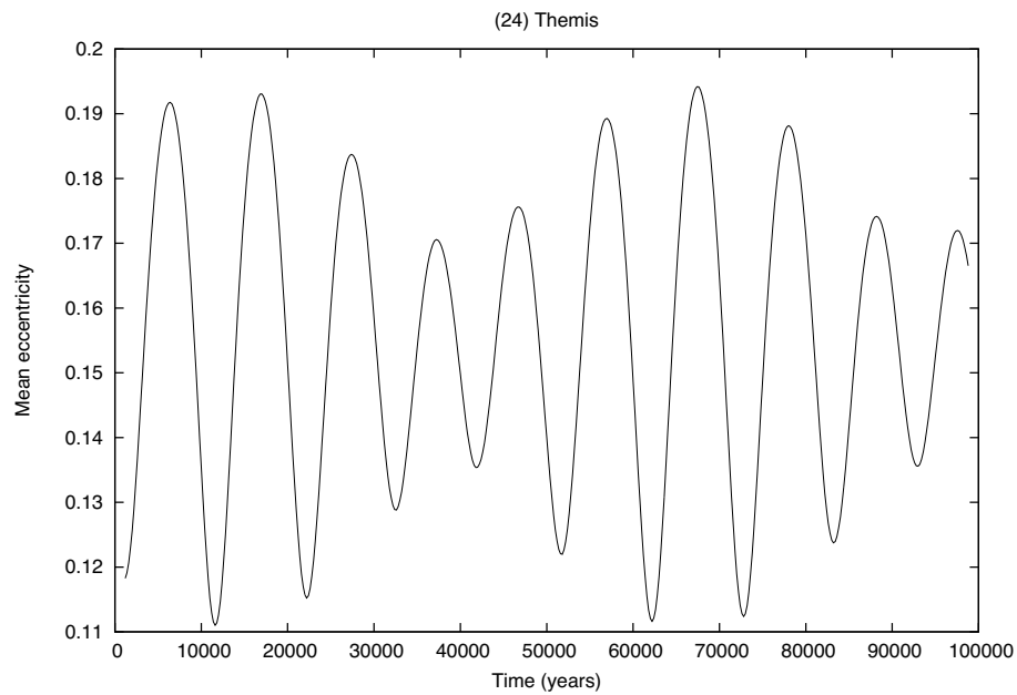
Figure 2.3: Mean eccentricity, computed by digital filtering, for the asteroid (24) Themis, as a function of time over 100 000 years.
