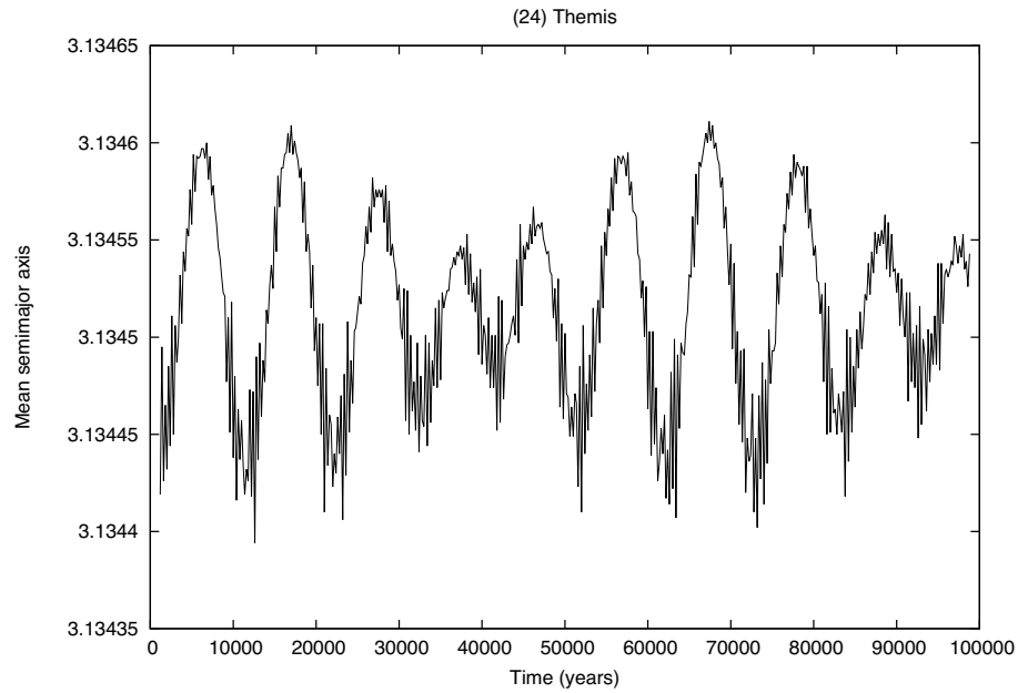
Figure 2.2: Mean semimajor axis, computed by digital filtering, for the asteroid (24) Themis, as a function of time over 100 000 years.
