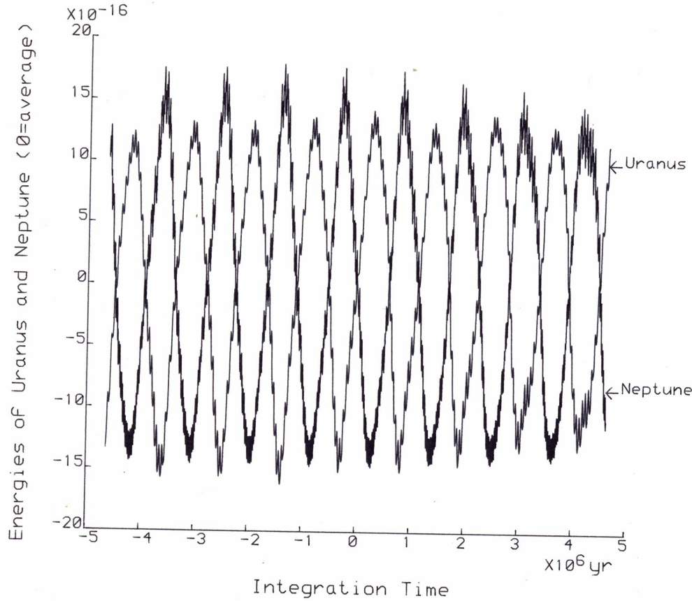
Figure 2.1: Energy of Uranus and Neptune over the 10 million years of the LONGSTOP 1A numerical integration (performed in 1984).
